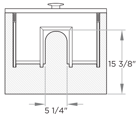
BOTTOM DRAWER top view
